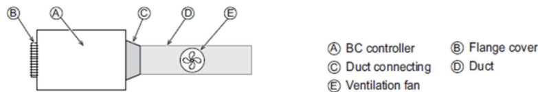
One BC controller to one ventilation fan (Mitsubishi App Note 2045, Fig. 7).
